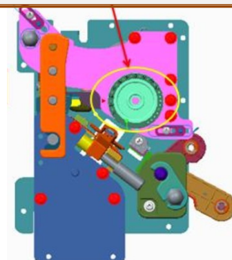
TPH module horizontal axis dial structure
